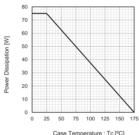
Fig.6 Power Dissipation
