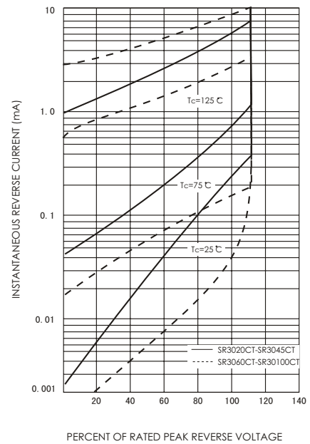
FIG.4-TYPICAL REVERSE CHARACTERISTICS
