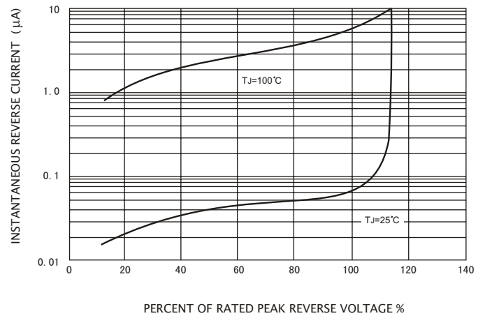
FIG.4-TYPICAL REVERSE CHARACTERISTICS
