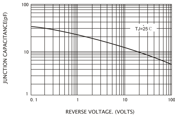
FIG.5-TYPICAL JUNCTION CAPACITANCE
