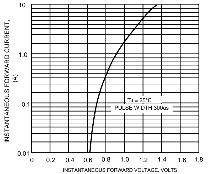
FIG.4-TYPICAL FORWARD CHARACTERISTICS
